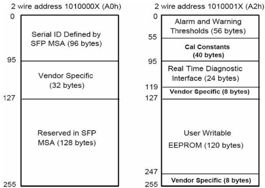
Digital Diagnostic Memory Map (Specific Data Field Descriptions)
