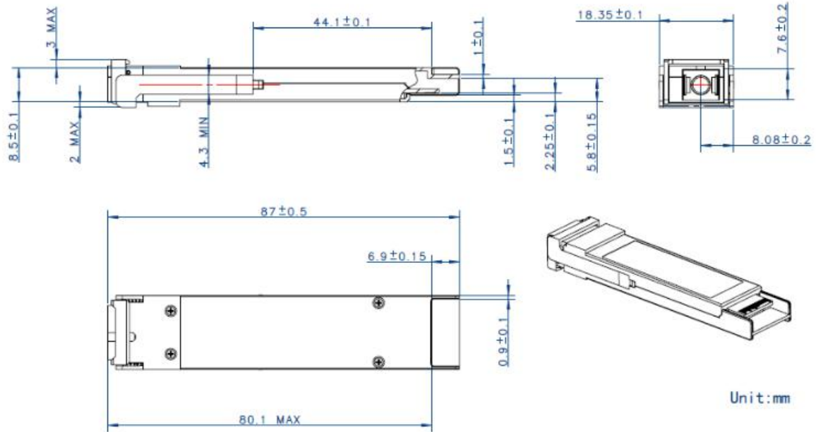
Figure 8: Package Outline
