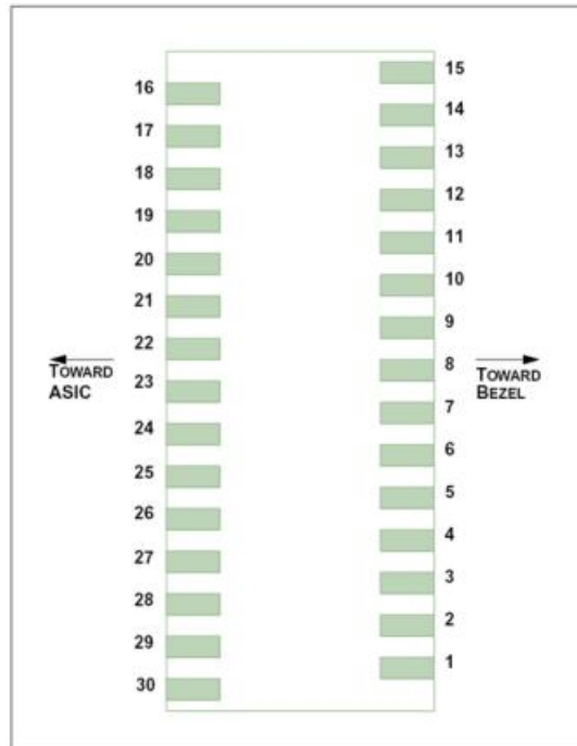
Figure 5: Pin Out Drawing
