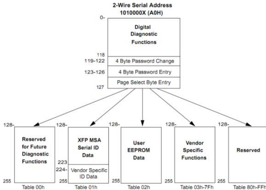
Figure 7: EEPROM Memory Map Specific Data Field Description
