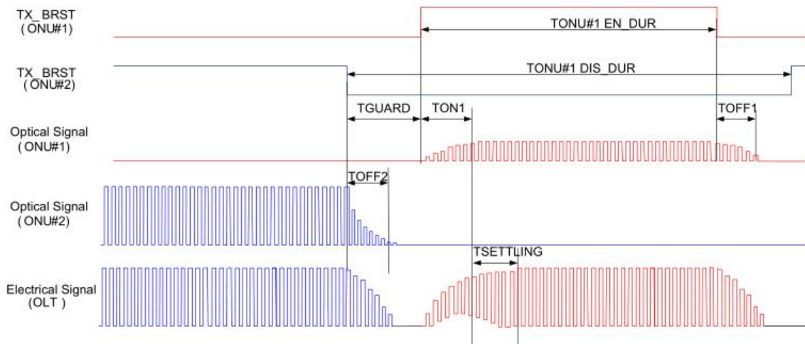
Figure 3: Timing Parameter Definitions in Burst Mode Sequence
